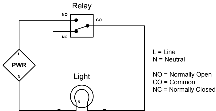
Figure 1: Normally Open Circuit
